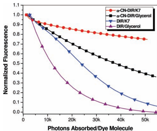
Figure 3. Photobleaching of DIR and \alpha -CN-DIR in 90% glycerol or in the presence of scFv K7. Samples were excited at 595 \pm 20 nm (DIR) and 540 \pm 12.5 nm ( \alpha -CN-DIR). Concentrations were adjusted to ensure initial equivalent absorbances at the excitation wavelength.
