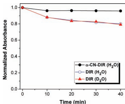
Figure 5. Reaction of K7-bound DIR and \alpha -CN-DIR with singlet oxygen produced by sodium molybdate and \text{H}_2\text{O}_2 . Reactions were run in buffer with [\text{dye}] = [\text{K7}] = 1 \mu\text{M} and \text{pH} = 9 , [\text{Na}_2\text{MoO}_4] = 50 \text{ mM} , [\text{H}_2\text{O}_2] = 9.8 \text{ mM} .
