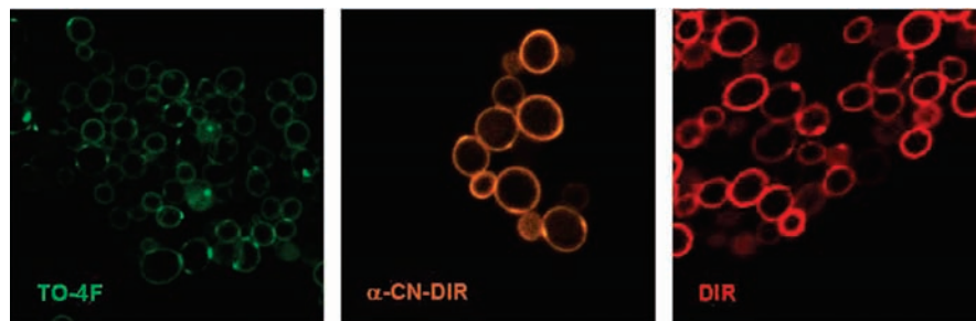
Figure 11. Confocal fluorescence micrographs of yeast-displayed scFv K7 stained with 300 nM TO-4F (left), 200 nM \alpha -CN-DIR (middle), and 100 nM DIR (red). (Fluorescence and differential interference contrast overlay images are shown in Supporting Information, Figure S3.)
