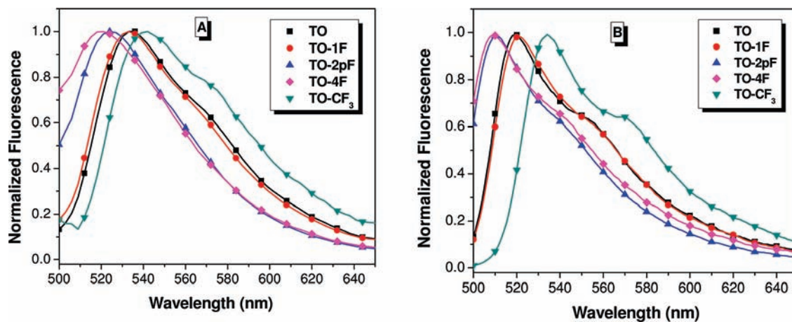
Figure 9. Fluorescence spectra of TO and fluorinated analogues bound to K7 protein displayed on the surface of yeast (A) or in solution (B). [Dye] = 300 nM in both cases. For A, 10^7 cells used. For B, 600 nM soluble K7 used. Samples were excited at 480 nm.
