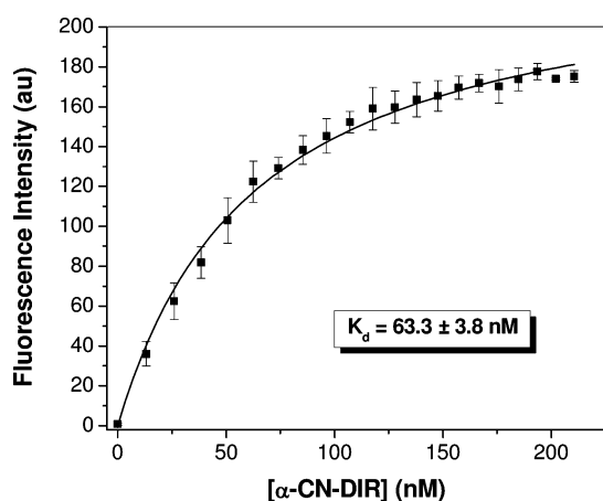
Figure 2. Binding of \alpha\text{-CN-DIR} to scFv K7 as shown by fluorescence titration. Samples contained 10 nM [K7] and were excited at 534 nm. Solid line is fit to a 1:1 binding model.
