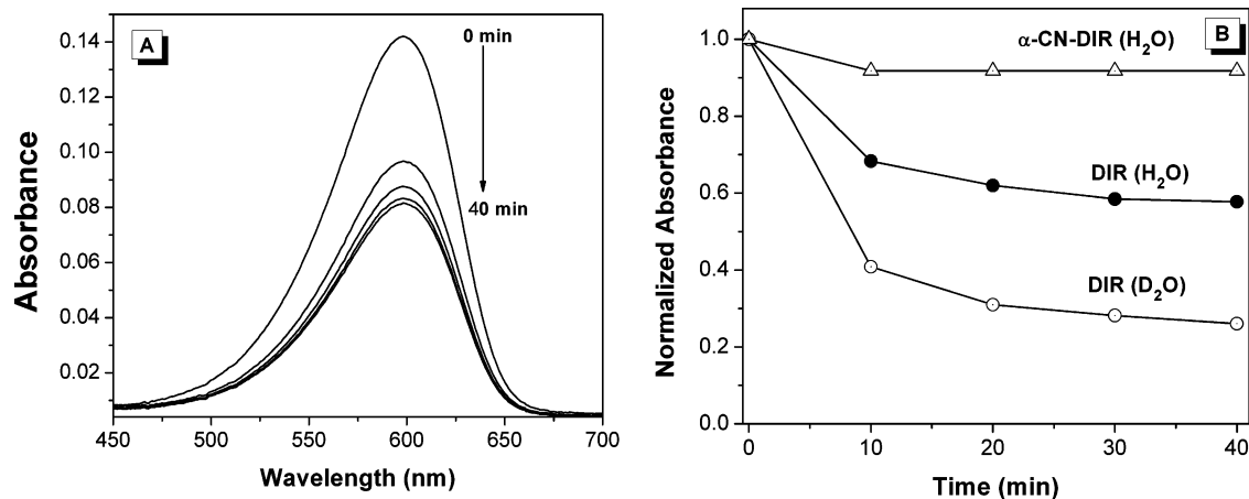
Figure 4. Reaction of DIR and \alpha -CN-DIR with singlet oxygen produced by sodium molybdate and \text{H}_2\text{O}_2 . Reactions were run in water with [\text{dye}] = 1 \mu\text{M} and \text{pH} = 9 , [\text{Na}_2\text{MoO}_4] = 50 \text{ mM} , [\text{H}_2\text{O}_2] = 9.8 \text{ mM} . (A) DIR absorbance spectra recorded in \text{H}_2\text{O} during reaction with \text{Na}_2\text{MoO}_4 and \text{H}_2\text{O}_2 . (B) Time course for dye bleaching for DIR in \text{H}_2\text{O} and \text{D}_2\text{O} as well as \alpha -CN-DIR in \text{H}_2\text{O} .
