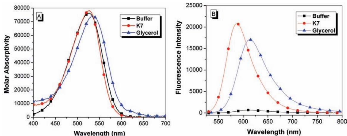
Figure 1. UV-vis absorption (A) and fluorescence emission spectra (B) recorded for 0.6 \mu\text{M} \alpha\text{-CN-DIR} in aqueous buffer (squares), 90% glycerol-in-water (triangles), and FAP K7 (circles). Samples in B were excited at 520 nm.
