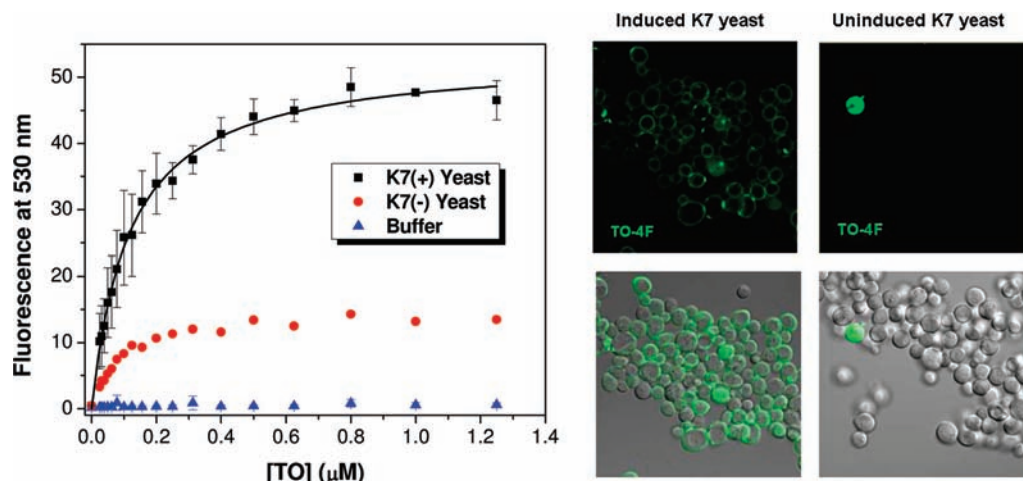
Figure 7. (Left) Fluorescence titration of TO into yeast-surface-displayed K7. Line is fit to a 1:1 binding model. Dye was titrated into yeast cells expressing K7 (squares), yeast not expressing K7 (circles), and buffer (triangles). Samples were excited at 480 nm. (Right) Confocal fluorescence microscope images of yeast stained with 300 nM TO-4F either with or without inducing expression of the surface-displayed K7 protein. Samples were excited at 488 nm, and fluorescence was collected at 517–583 nm. Bottom panels show merge of fluorescence and differential interference contrast images.
