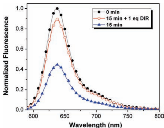
Figure 6. Photobleaching of DIR/K7 by direct irradiation at \lambda > 455 \text{ nm} for 15 min. Initial [\text{DIR}] = [\text{K7}] = 250 \text{ nM} . Fluorescence emission spectra ( \lambda_{\text{ex}} = 590 \text{ nm} ) were recorded before and after 15 min irradiation. After irradiation, 1 equiv of fresh DIR was added to the cuvette and the fluorescence spectrum was recorded.
